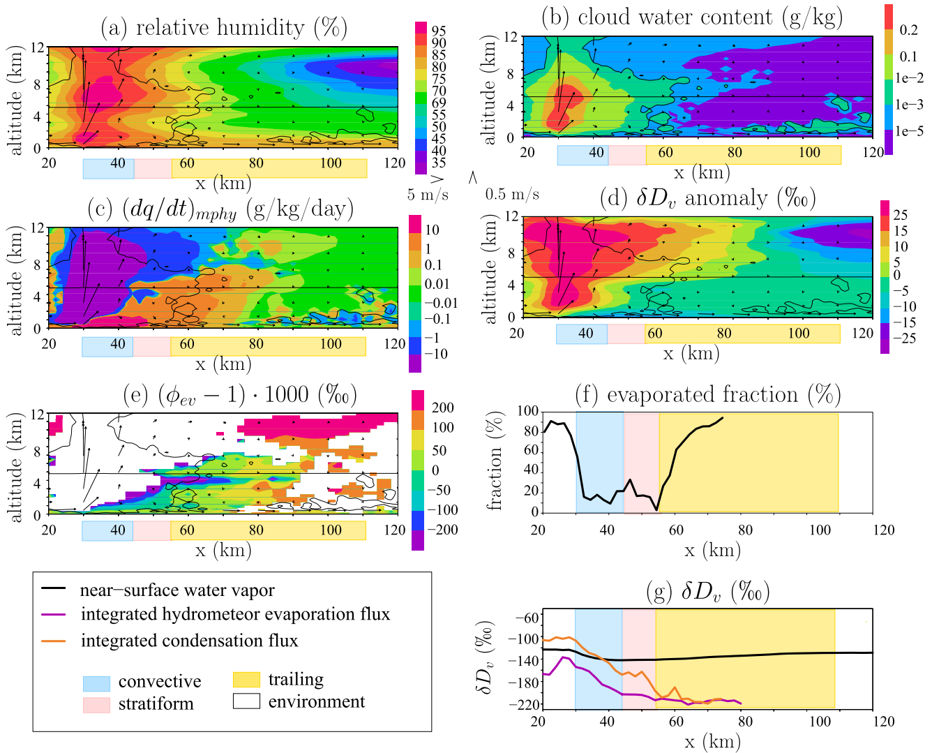
Figure 8. Same as Figure 5, except that variables for the squall line simulation are shown as a function of the distance along the x -axis. The blue, pink, and yellow boxes indicate the convective, stratiform, and trailing regions defined in Section 3.2.2.
