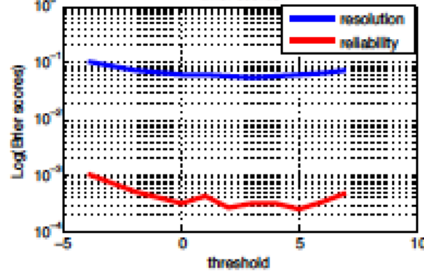
Brier scores
