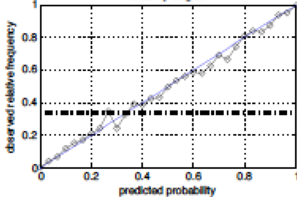
reliability diagram
