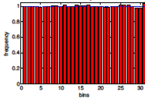
rank histogram
