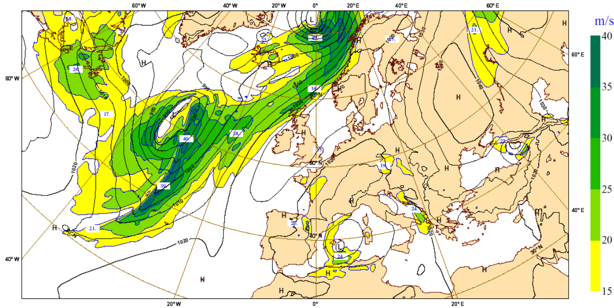
Monday 7 November 2011 00UTC ©ECMWF Analysis t+000 VT: Monday 7 November 2011 00UTC Surface: Mean sea level pressure / 850-hPa wind speed
