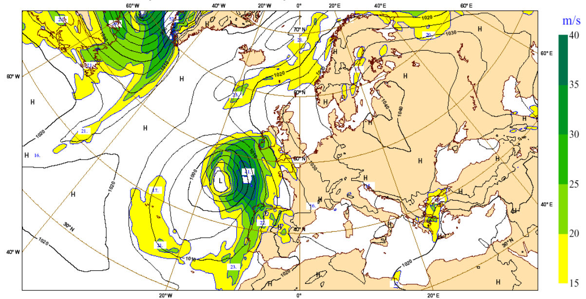
Sunday 13 November 2011 00UTC ©ECMWF Analysis t+000 VT: Sunday 13 November 2011 00UTC Surface: Mean sea level pressure / 850-hPa wind speed
