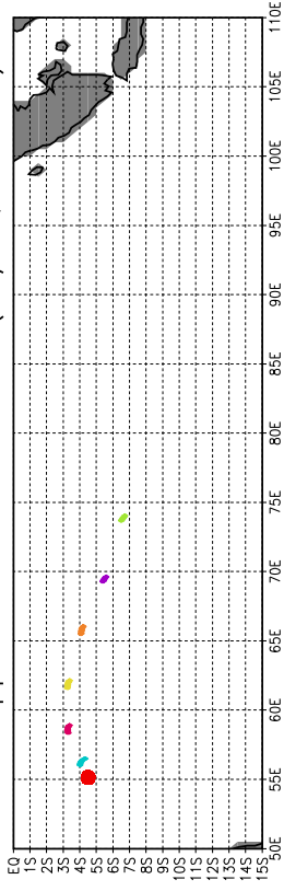
Aeroclippers laches a J+78 h (25/12, 18 UTC)
