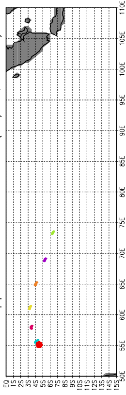
Aeroclippers laches a J+90 h (26/12, 6 UTC)
