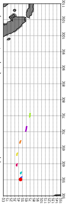
Aeroclippers laches a J+60 h (25/12, 00 UTC)
