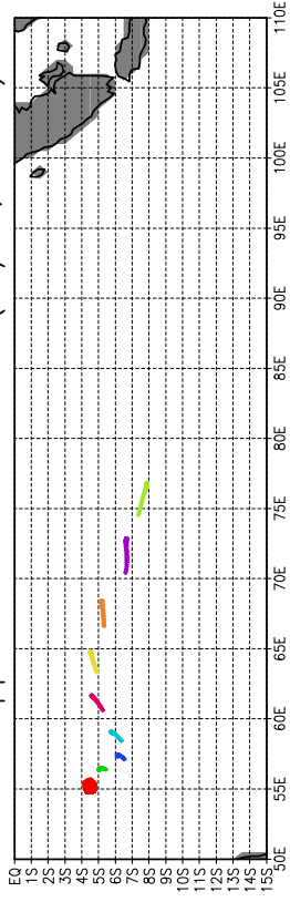
Aeroclippers laches a J+18 h (23/12, 6 UTC)
