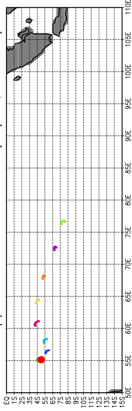
Aeroclippers laches a J+48 h (24/12, 12 UTC)
