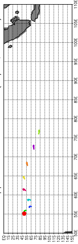
Aeroclippers laches a J+36 h (24/12, 00 UTC)
