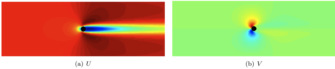
Figure 2.3: U, V velocity components for flow around a cylinder, courtesy of P.J. Schmid.
