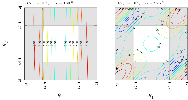
Figure 4.5: Contours of the amplification factor for the convection-diffusion problem, for a mesh-based Reynolds number of Re_h = 10^2 . Upstream marching is used. Comparison with the bottom right plot in Figure 4.4, where downstream marching has been used, shows a strong degradation, by two orders of magnitude, in the amplification factor for both U = -1, V = 0 ( \alpha = -180^\circ , left plot) and for U = V = -1/\sqrt{2} ( \alpha = -135^\circ , right plot). The sweep direction is paramount in regions of the computational domain with high mesh-based Reynolds numbers. The corresponding symbol is given by (4.39).
