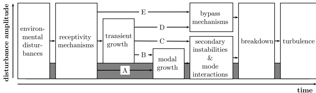
Figure 1.2: Transition mechanisms. Different mechanisms can be responsible for transition from laminar to turbulent flow, but at the origin there is the concept of receptivity: incoming disturbances from the environment — e.g. variations in the incoming free stream — enter the boundary layer and trigger the development of perturbations. These perturbations may then be amplified by different mechanisms, like modal growth or transient growth, may lead to secondary instabilities and/or cause transition to turbulence. A correct understanding of the perturbation behavior and of the receptivity mechanism is essential for increasing the extent of the laminar flow regime in boundary layers by applying control techniques.
