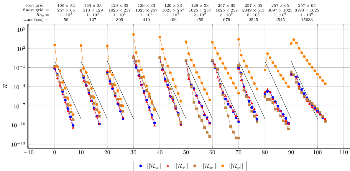
Figure 5.1: Convergence behavior for the computation of base flows at different Reynolds numbers. Residuals are shown for the discrete u, v, w -momentum and pressure equations separately, and the continuous black line represents the theoretical convergence estimate for the Poisson equation of 0.125 per V-cycle. Each mark in the series represents a V-cycle of the multigrid solver with two linewise Gauss-Seidel relaxation sweeps on the downward leg and one sweep on the upward leg. The last computation on the right includes adaptive grid refinement: the finest grid covers only part of the computational domain covered by the coarser one.
