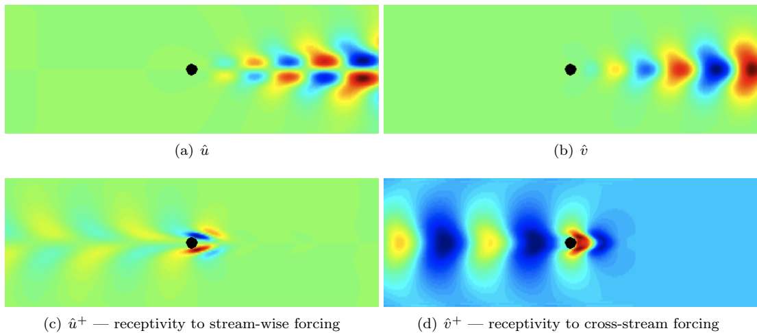
Figure 2.4: Direct and adjoint fields for a cylinder wake, courtesy of P.J. Schmid.
