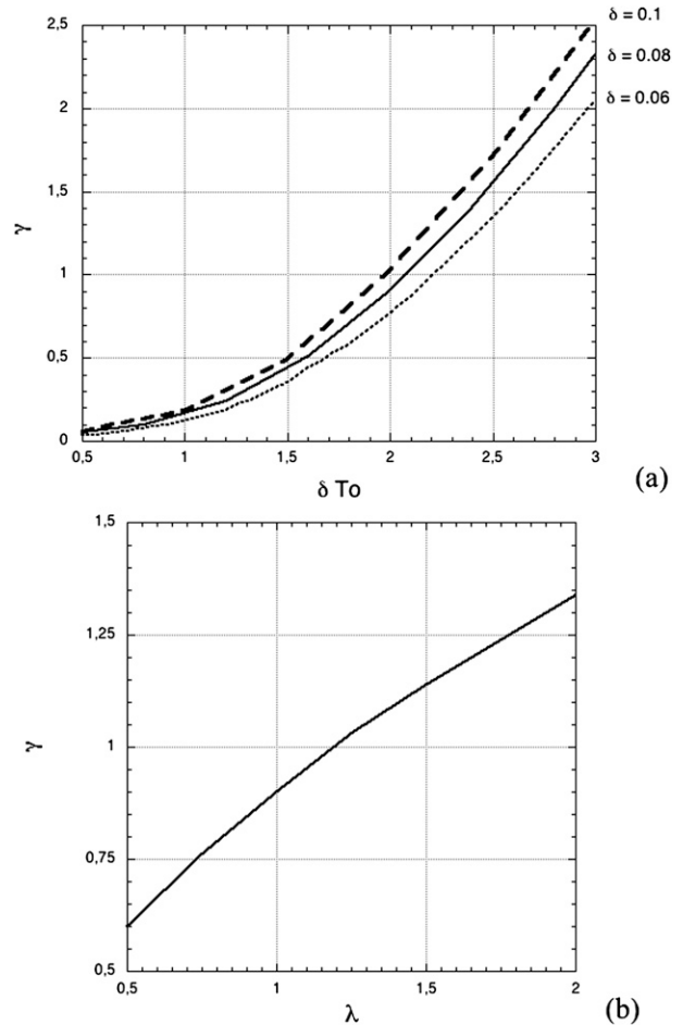
FIG. 6. Evolution of the acceleration coefficient \gamma (a) as a function of the product \delta To (for the following values of \delta : 0.06, 0.08, and 0.1) and (b) as a function of the relative isopycnal deviation parameter \lambda .
