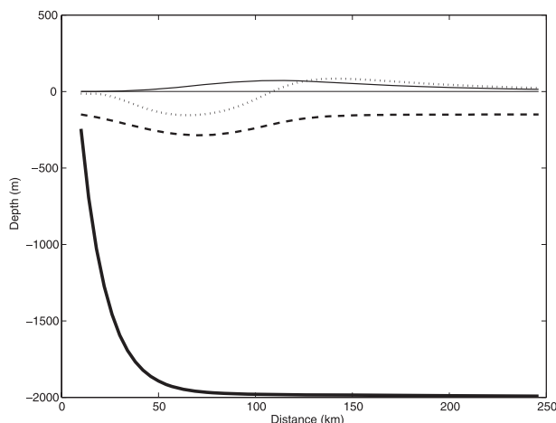
FIG. 8. The cross-isobath profiles of the ocean depth (thick line), upper-layer interface (dashed line), lower-layer geopotential (thin line), and corresponding alongshore velocity (dotted line) after six months of integration.
